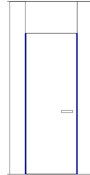
Porta pivot con soprapporta 20mm Pivot door with transom panel 20mm H 1800 / 3200 L 700 / 1500
