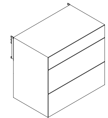
3 Cassetti in legno 3 Wooden drawers H 733 - P 540 L 600 - 900 - 1200
