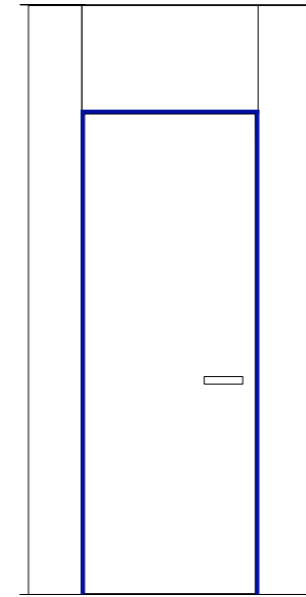
Porta a battente con soprapporta 20mm Swing door with transom panel 20mm H 1800 / 3200 L 600 / 1200
