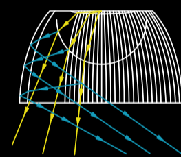
Materic convergence between lens and antiglare Optical PMMA
